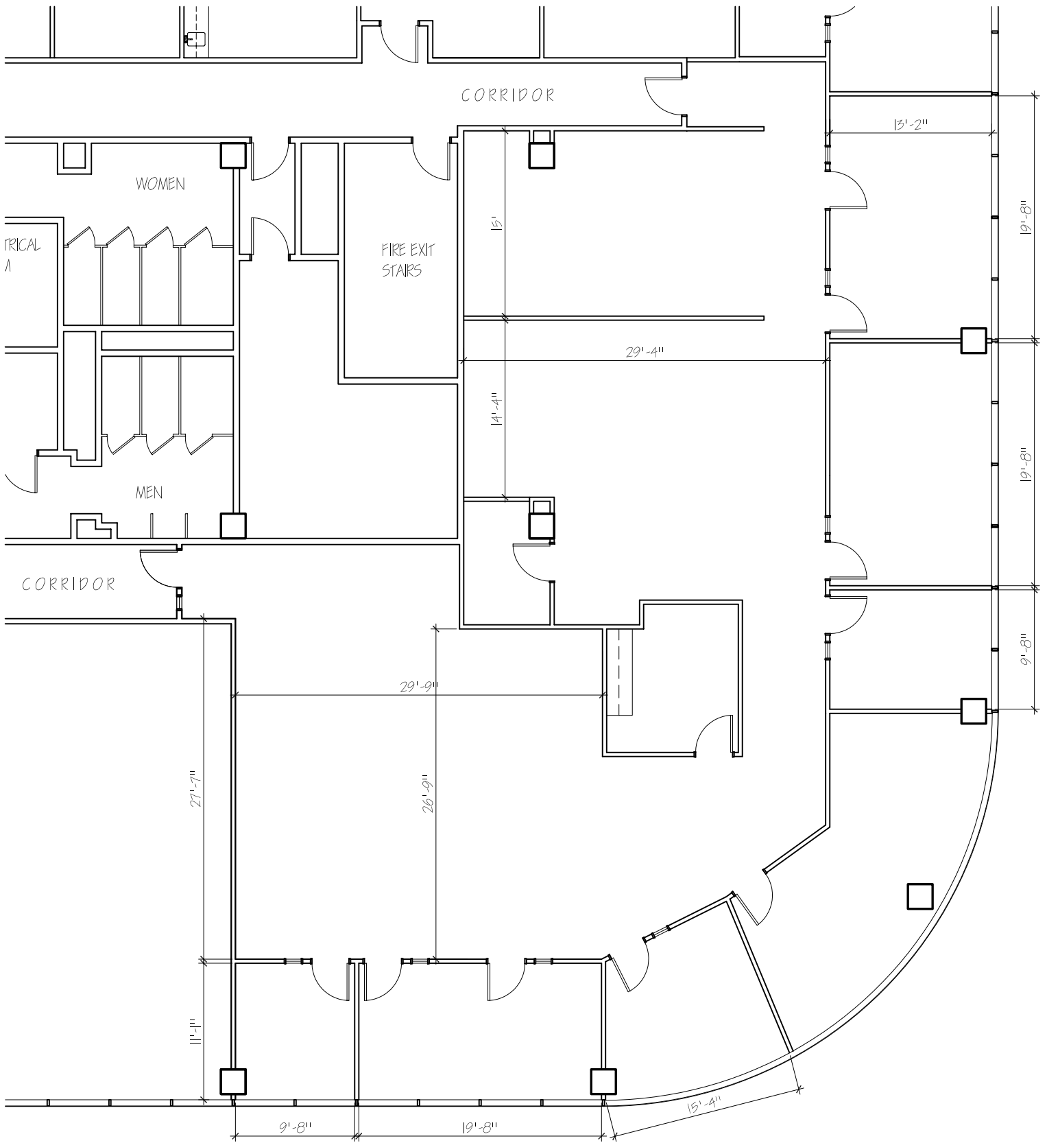
Suite #600 - Existing Floor Plan 3530 Wilshire Blvd. Scale: 3/32" = 1'-0"
