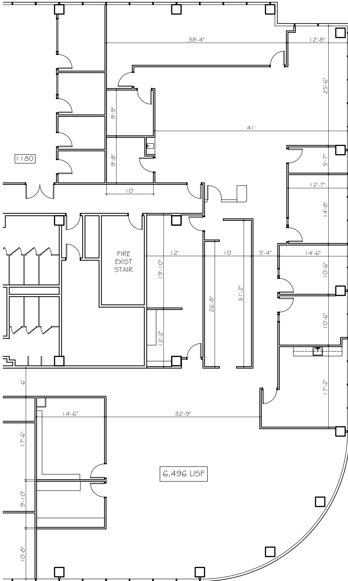
SUITE #1110 - EXISTING FLOOR PLAN 3530 Metroplex, Wilshire Blvd.
