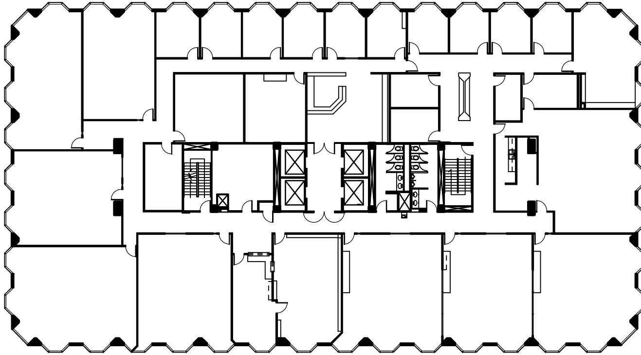
SECOND FLOOR-NORTH
